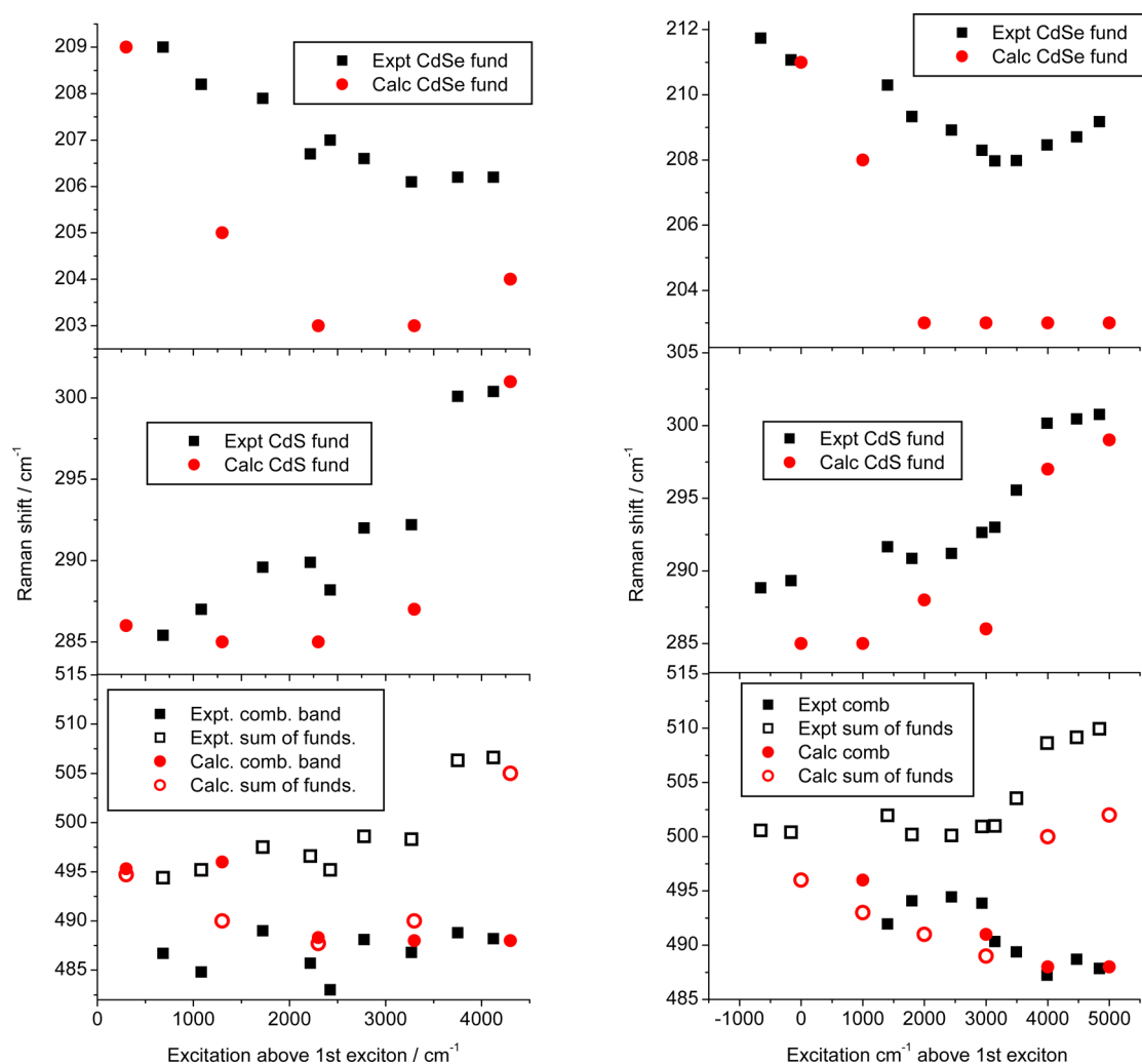
Figure 7. Experimental (black) and calculated (red) frequencies for CdSe fundamental (top), CdS fundamental (middle), and CdSe + CdS combination band (bottom), for thin-shelled (left) and thick-shelled (right) CdSe/CdS QDs. Open symbols in bottom plot are the sum of the fundamental peak frequencies.
